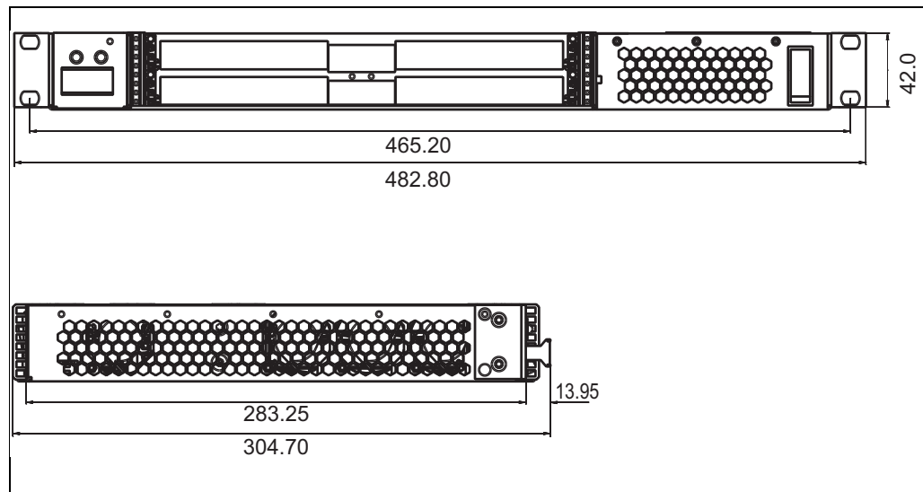
Figure 5: Maße
